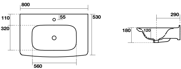
5641 Lavabo cm 80 Washbasin cm 80
