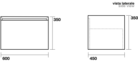
9151 Mobile sospeso cm 60 con cassetto Wall hung cabinet cm 60 with drawer
