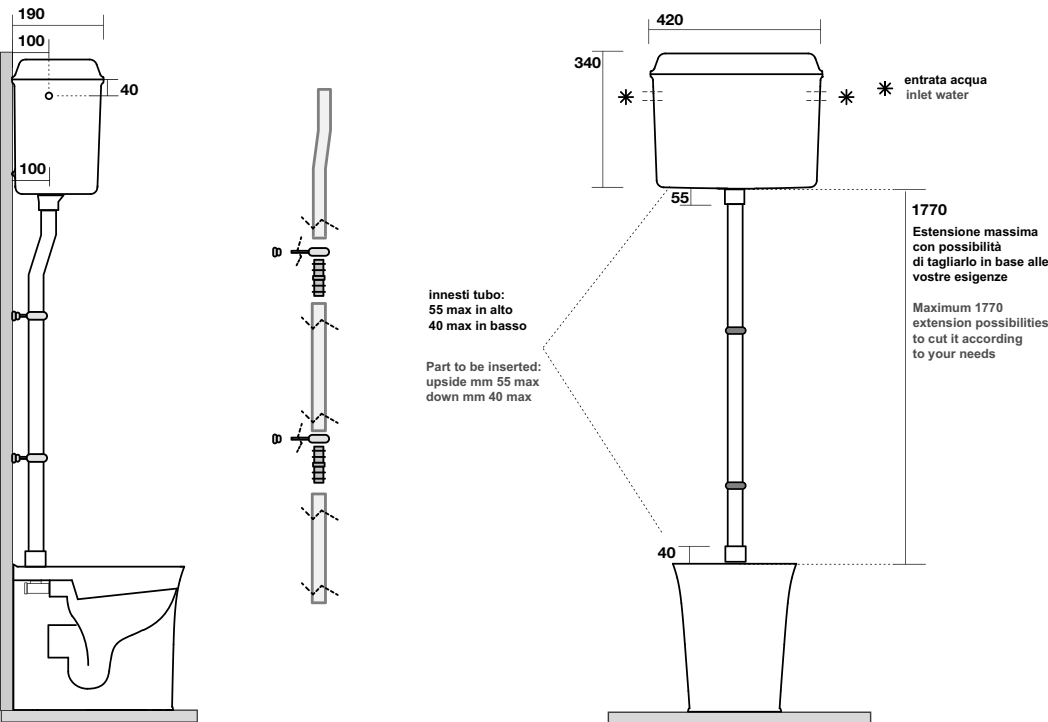
5680 Cassetta alta High level cistern
