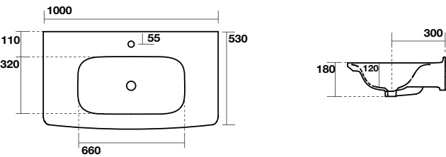
5642 Lavabo cm 100 Washbasin cm 100
