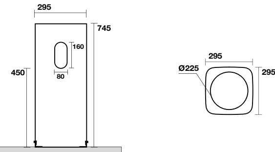
5574 OKE colonna scarico a parete per Art. 5541 OKE pedestal wall drain for Art. 5541
